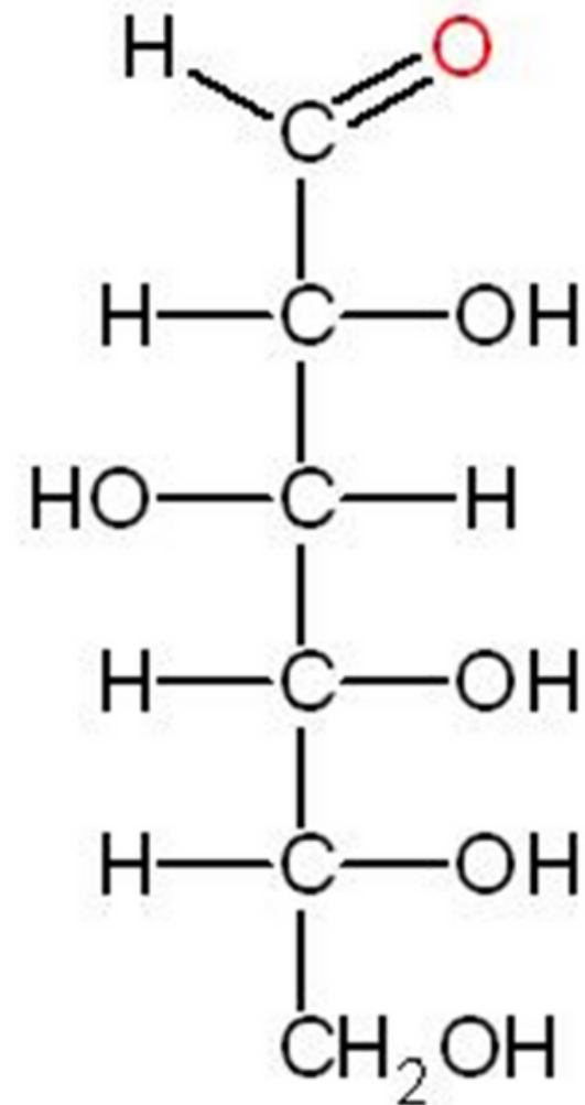
D-glucose
