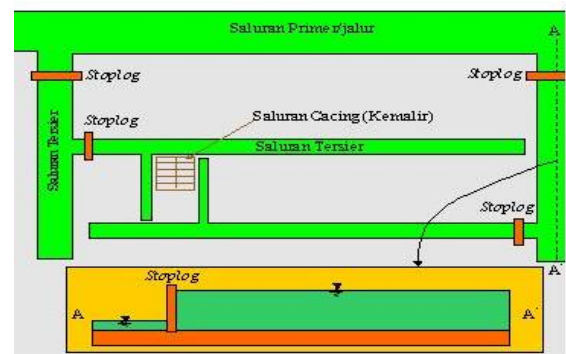
Gambar 3. Sistem Tata Air di Lahan Gambut (Haerani & Nursyamsi, 2012)
