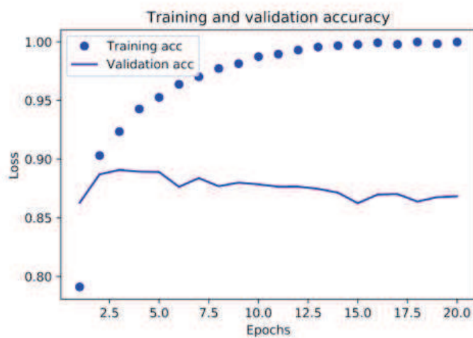
Figure 3.8 Training and validation accuracy
