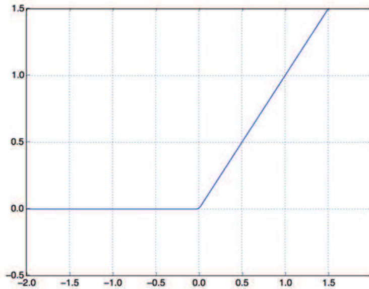
Figure 3.4 The rectified linear unit function
