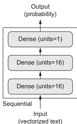
Figure 3.6 The three-layer network
