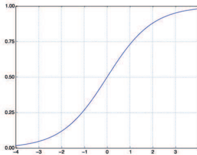
Figure 3.5 The sigmoid function
