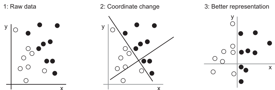
Figure 1.4 Coordinate change
