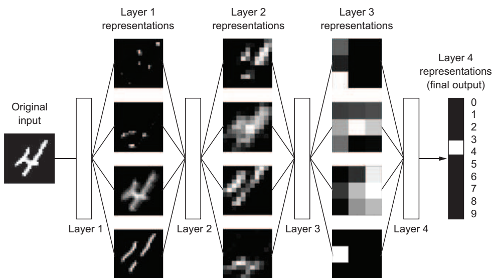
Figure 1.6 Deep representations learned by a digit-classification model
