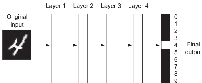
Figure 1.5 A deep neural network for digit classification
