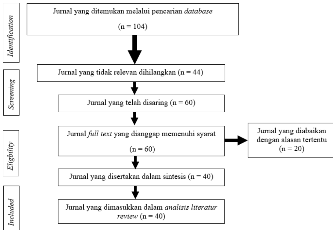
Gambar 1 Diagram PRISMA
