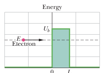
Figure 38-17 An energy diagram containing two plots for the situation of Fig. 38-16: (1) The electron's mechanical energy E is plotted when the electron is at any coordinate x < 0 . (2) The electron's electric potential energy U is plotted as a function of the electron's position x , assuming that the electron can reach any value of x . The nonzero part of the plot (the potential barrier) has height U_b and thickness L .
