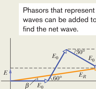
Figure 35-14 Three phasors, representing waves with equal amplitudes E_0 and with phase constants 0^\circ , 60^\circ , and -30^\circ , shown at time t = 0 . The phasors combine to give a resultant phasor with magnitude E_R , at angle \beta .
