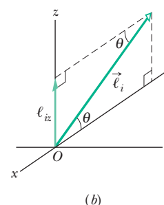
Figure 11-15 (a) A rigid body rotates about a z axis with angular speed \omega . A mass element of mass \Delta m_i within the body moves about the z axis in a circle with radius r_{\perp i} . The mass element has linear momentum \vec{p}_i , and it is located relative to the origin O by position vector \vec{r}_i . Here the mass element is shown when r_{\perp i} is parallel to the x axis. (b) The angular momentum vector \vec{\ell}_i , with respect to O , of the mass element in (a). The z component \ell_{iz} is also shown.
