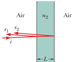
Figure 35-17 Reflections from a thin film in air.
