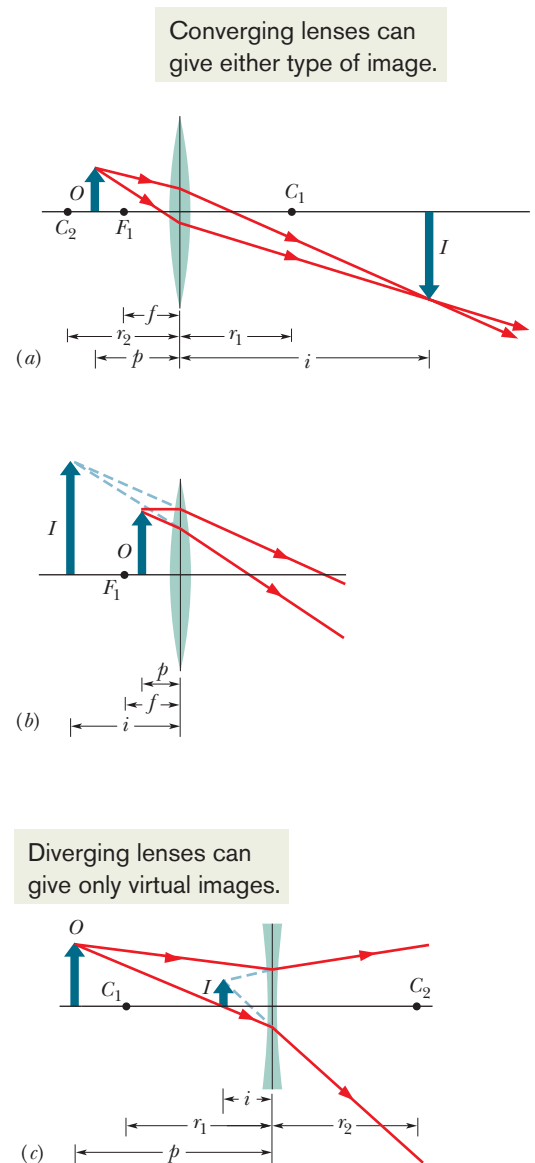
Figure 34-15 (a) A real, inverted image I is formed by a converging lens when the object O is outside the focal point F_1 . (b) The image I is virtual and has the same orientation as O when O is inside the focal point. (c) A diverging lens forms a virtual image I , with the same orientation as the object O , whether O is inside or outside the focal point of the lens.
