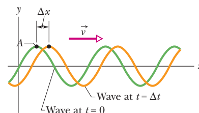
Figure 16-7 Two snapshots of the wave of Fig. 16-4, at time t = 0 and then at time t = \Delta t . As the wave moves to the right at velocity \vec{v} , the entire curve shifts a distance \Delta x during \Delta t . Point A “rides” with the wave form, but the string elements move only up and down.
