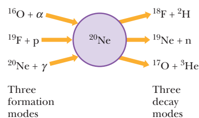
Figure 42-14 The formation modes and the decay modes of the compound nucleus ^{20}\text{Ne} .
