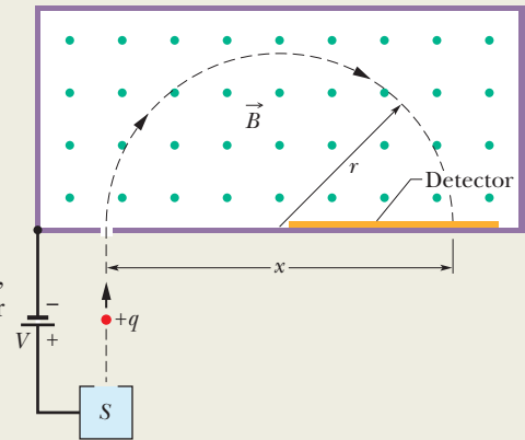
Figure 28-12 A positive ion is accelerated from its source S by a potential difference V , enters a chamber of uniform magnetic field \vec{B} , travels through a semicircle of radius r , and strikes a detector at a distance x .
