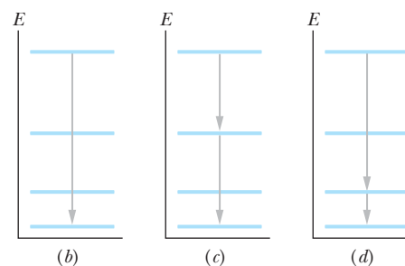
Figure 39-4 (a) Excitation of a trapped electron from the energy level of its ground state to the level of its third excited state. (b)–(d) Three of four possible ways the electron can de-excite to return to the energy level of its ground state. (Which way is not shown?)
