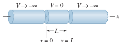
Figure 39-1 The elements of an idealized “trap” designed to confine an electron to the central cylinder. We take the semi-ininitely long end cylinders to be at an infinitely great negative potential and the central cylinder to be at zero potential.
