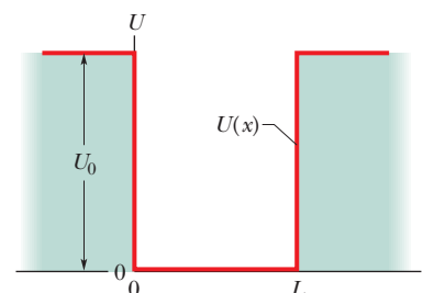
Figure 39-7 A finite potential energy well. The depth of the well is U_0 and its width is L . As in the infinite potential well of Fig. 39-2, the motion of the trapped electron is restricted to the x direction.
