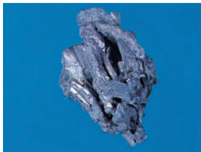
Arsenic (As)
