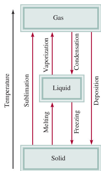
Figure 12.31 The various phase changes that a substance can undergo.
