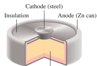
Electrolyte solution containing KOH and paste of \text{Zn}(\text{OH})_2 and \text{HgO}
