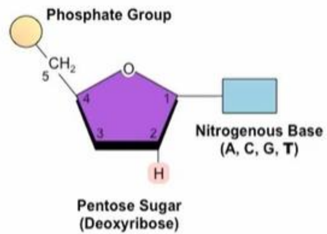
DNA Nucleotide
