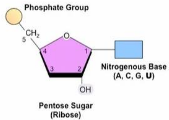
RNA Nucleotide
